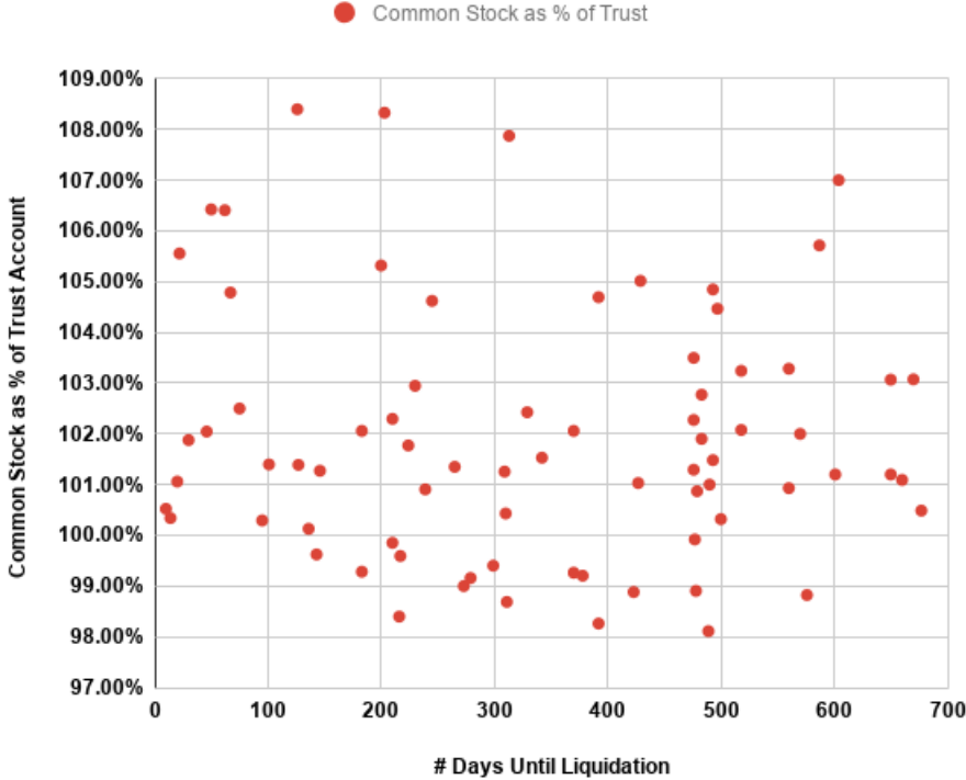
Common Stock as % of Trust vs. Time Remaining SPACs Without Definitive Agreement (07/15/2020)
